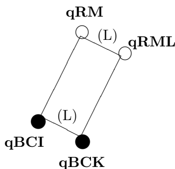
Figure 3: Hierarchy 2
