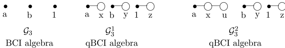
Figure 7: The p-semisimple BCI algebra \mathcal{G}_3 and the associated p-semisimple qBCI algebras \mathcal{G}_3^1, \mathcal{G}_3^2
