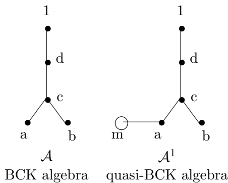
Figure 8: The regular BCK algebra \mathcal{A} and an associated quasi-BCK algebra, \mathcal{A}^1
