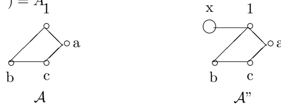
Figure 5: The Hasse-type diagram of the regular RML algebra \mathcal{A} and the quasi-Hasse-type diagram of the quasi-RML algebra \mathcal{A}''
